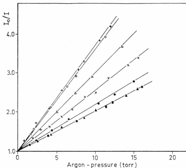
Fig. 3. Stern-Volmer plots of the (B \rightarrow A) fluorescence as a function of Ar pressure for different CO pressures; \blacktriangle p_{\text{CO}} = 0.7 mtorr, \blacksquare p_{\text{CO}} = 1.1 mtorr, \bullet p_{\text{CO}} = 4.8 mtorr, \times p_{\text{CO}} = 12 mtorr, \triangle p_{\text{CO}} = 24 mtorr, \circ p_{\text{CO}} = 38 mtorr, + p_{\text{CO}} = 56 mtorr.
