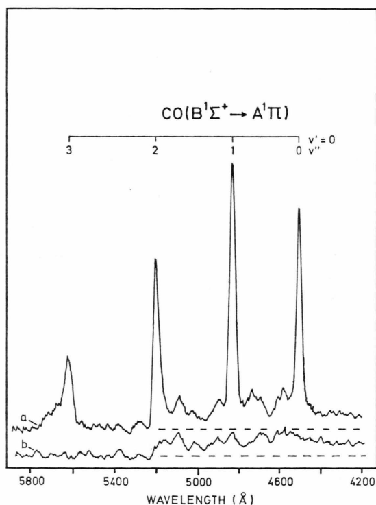
Fig. 1. Fluorescence spectrum of CO excited by a CO 2 /He microwave discharge lamp; trace a: p_{\text{CO}} = 50 mtorr, trace b: straylight spectrum.
